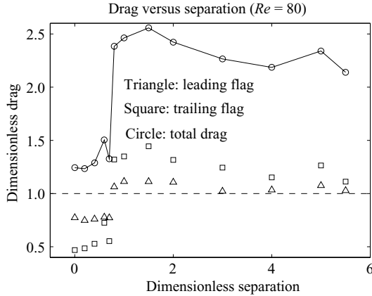
FIGURE 8. Drag versus separation distance for Re=80 . The x -axis is the flag separation distance D (dimensionless). The y -axis is the dimensionless drag. The dashed line represents the drag of a single flag. The triangles represent drag of the upper flag, the squares represent drag of the lower flag and circles represent the total drag of the flags.
